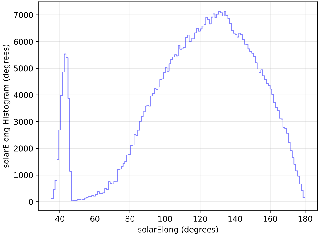
too_elab_heavy_r128_d2_gz_v3.4_10yrs WFD i band: solarElong Histogram
