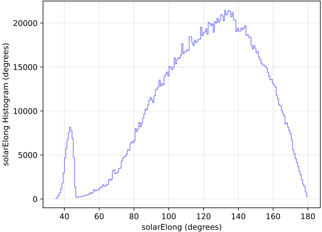
too_elab_heavy_r128_d2_gz_v3.4_10yrs WFD all bands: solarElong Histogram
