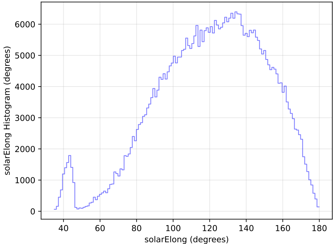
too_elab_heavy_r128_d2_gz_v3.4_10yrs All sky z band: solarElong Histogram
