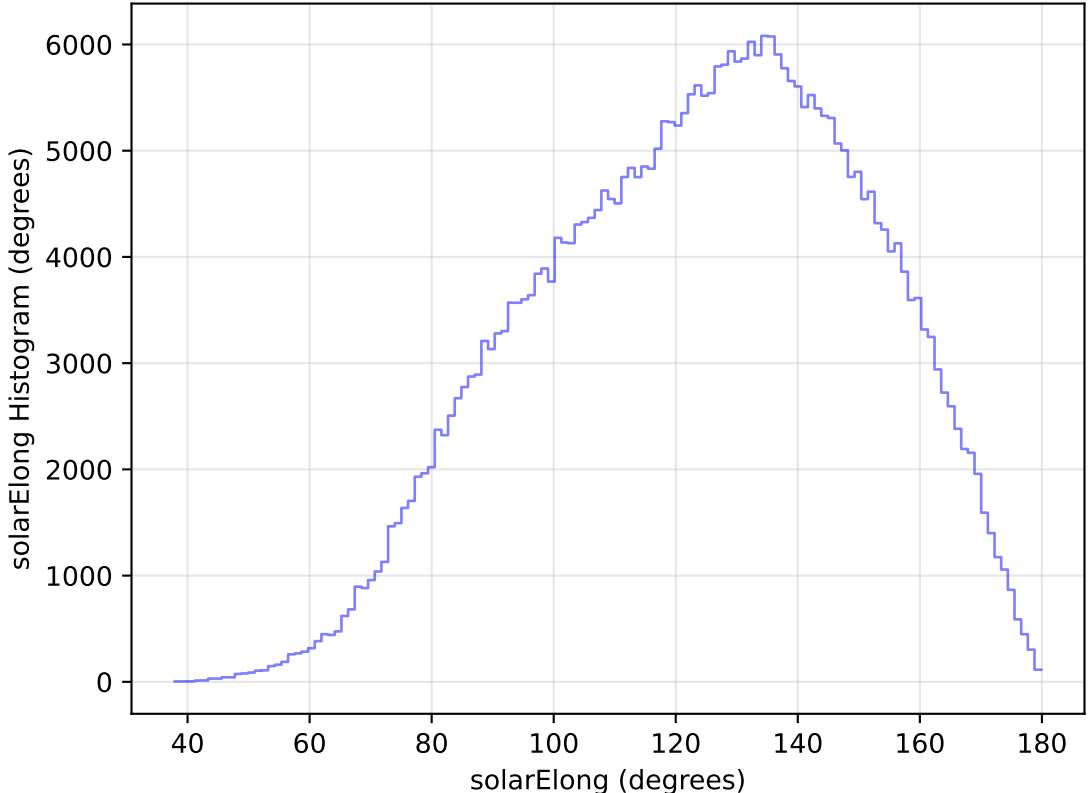
too_elab_heavy_r128_d2_gz_v3.4_10yrs All sky y band: solarElong Histogram
