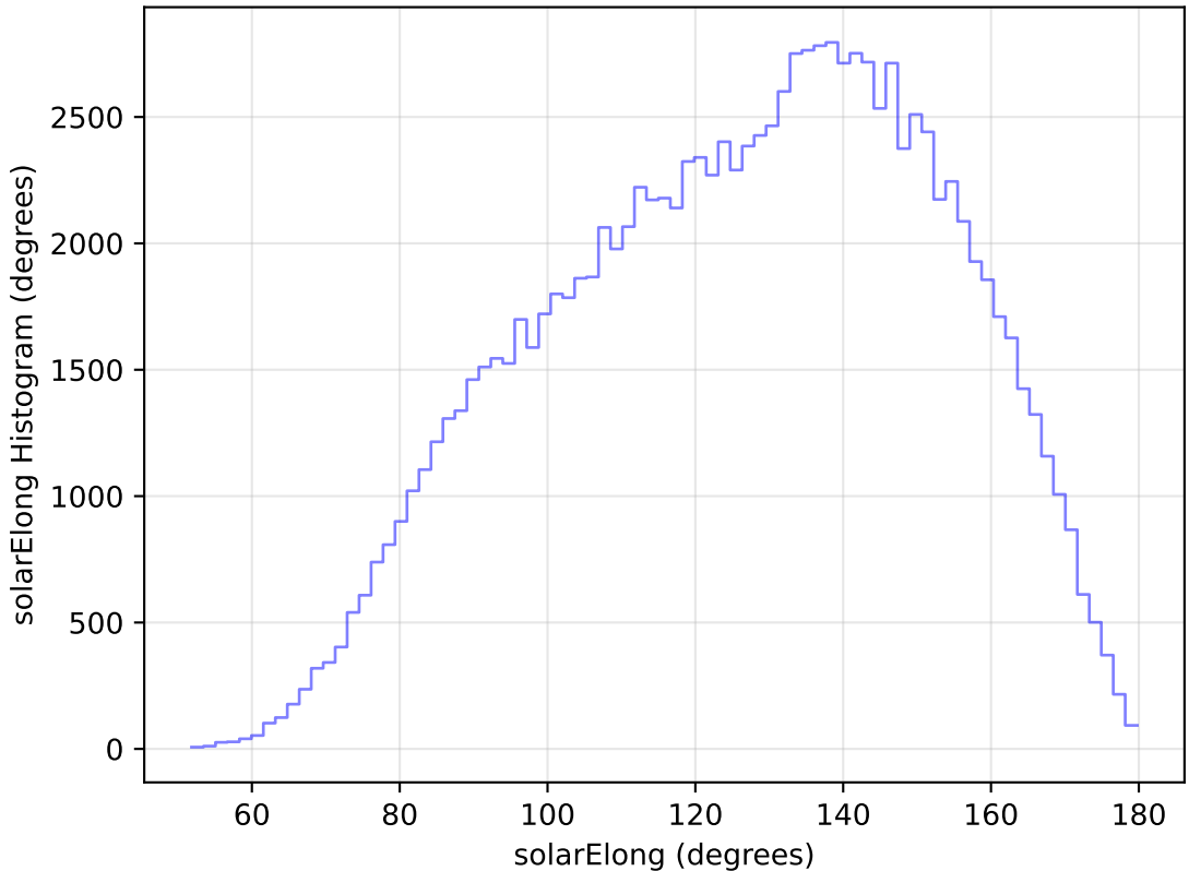
too_elab_heavy_r128_d2_gz_v3.4_10yrs All sky u band: solarElong Histogram
