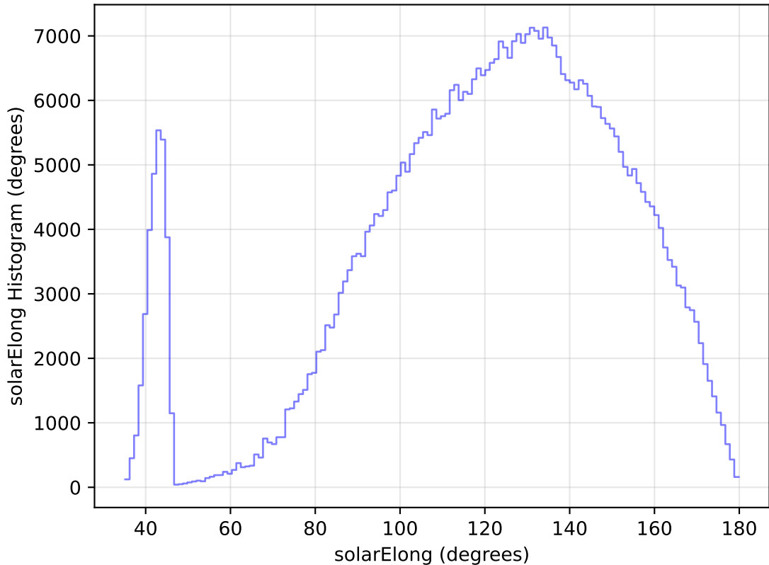
too_elab_heavy_r128_d2_gz_v3.4_10yrs All sky i band: solarElong Histogram
