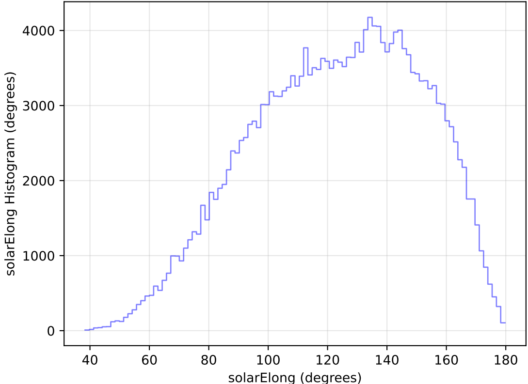
too_elab_heavy_r128_d2_gz_v3.4_10yrs All sky g band: solarElong Histogram
