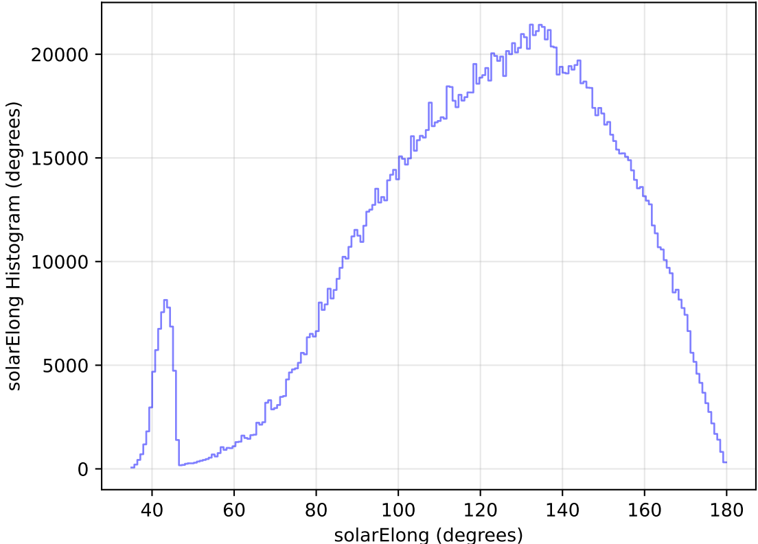
too_elab_heavy_r128_d2_gz_v3.4_10yrs All sky all bands: solarElong Histogram
