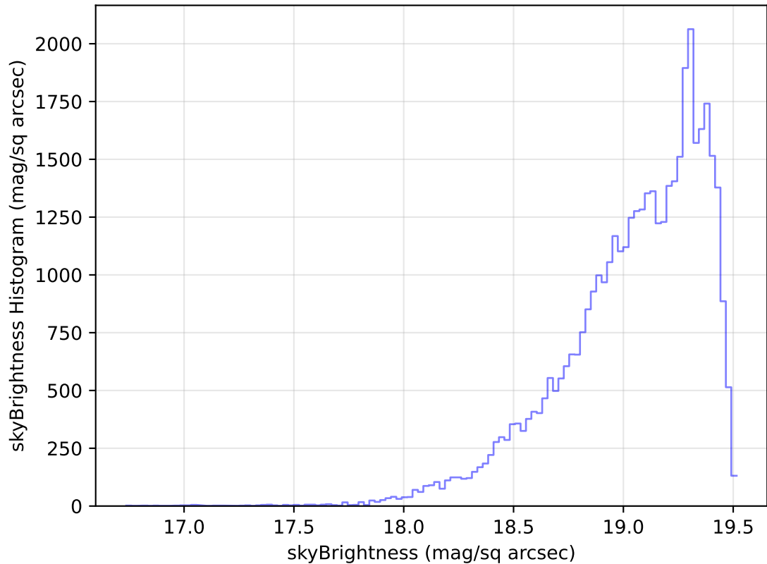
too_elab_heavy_r128_d2_gz_v3.4_10yrs Yr 1 z band: skyBrightness Histogram
