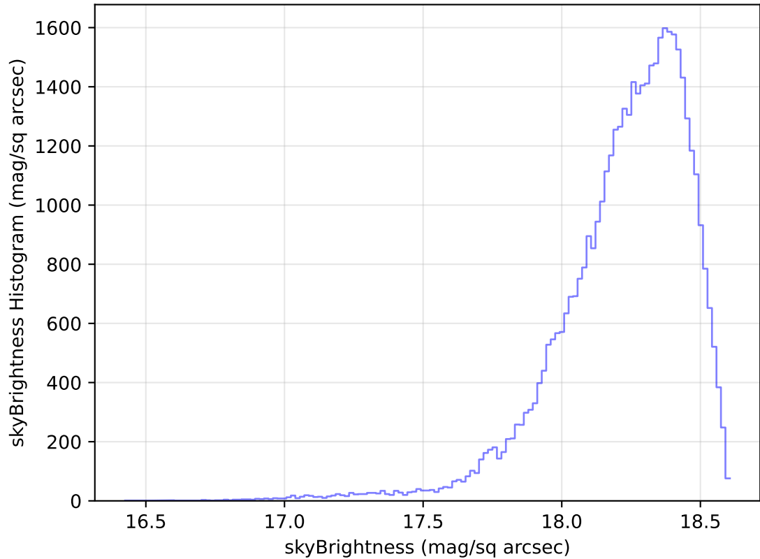
too_elab_heavy_r128_d2_gz_v3.4_10yrs Yr 1 y band: skyBrightness Histogram
