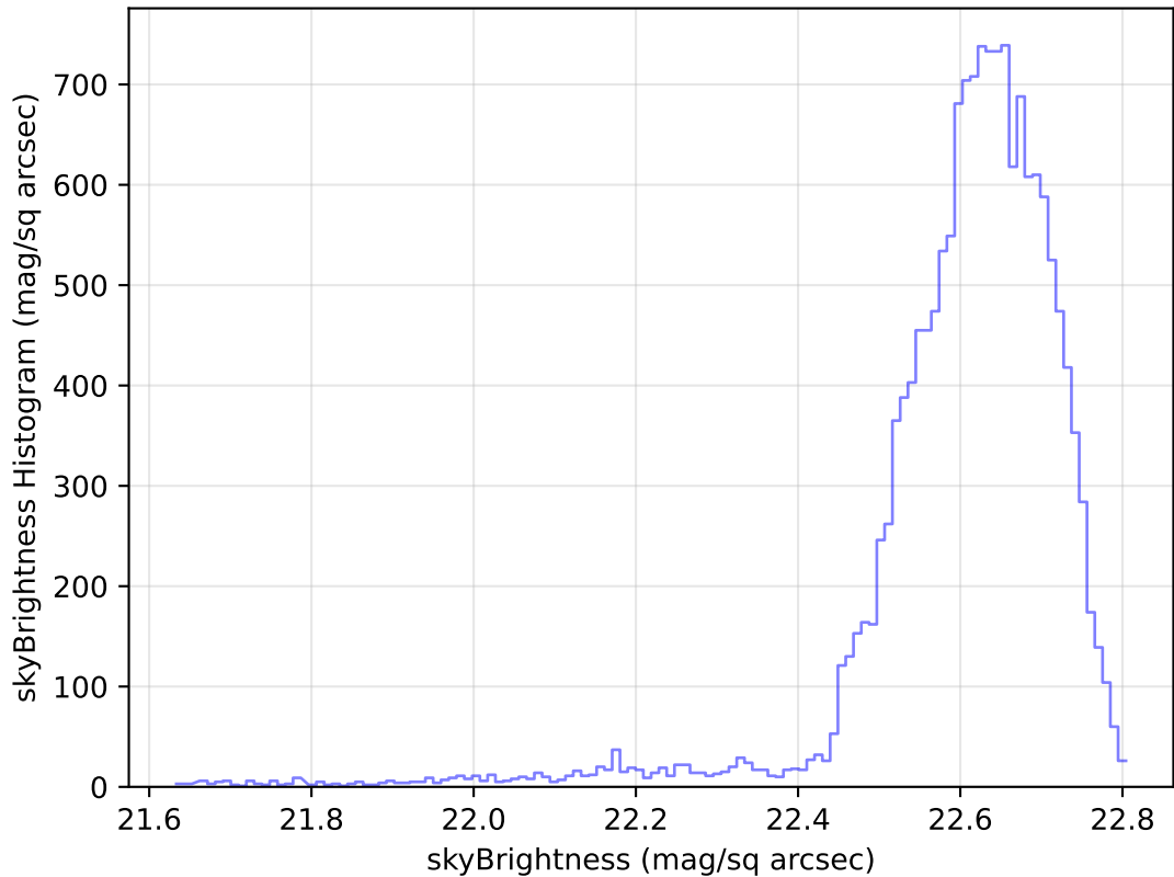
too_elab_heavy_r128_d2_gz_v3.4_10yrs Yr 1 u band: skyBrightness Histogram
