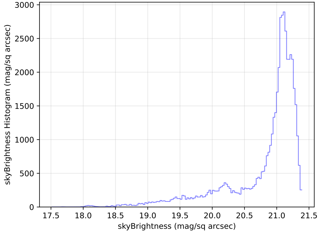
too_elab_heavy_r128_d2_gz_v3.4_10yrs Yr 1 r band: skyBrightness Histogram
