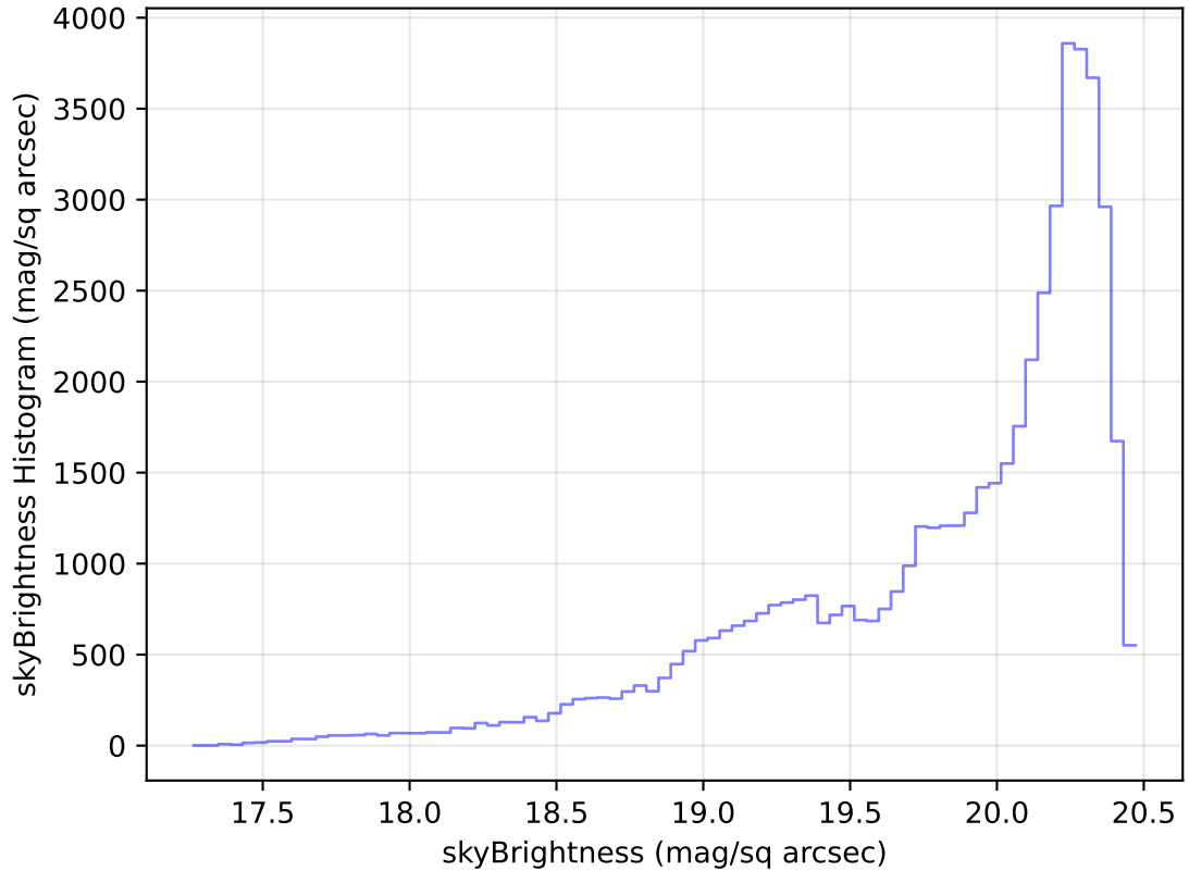
too_elab_heavy_r128_d2_gz_v3.4_10yrs Yr 1 i band: skyBrightness Histogram
