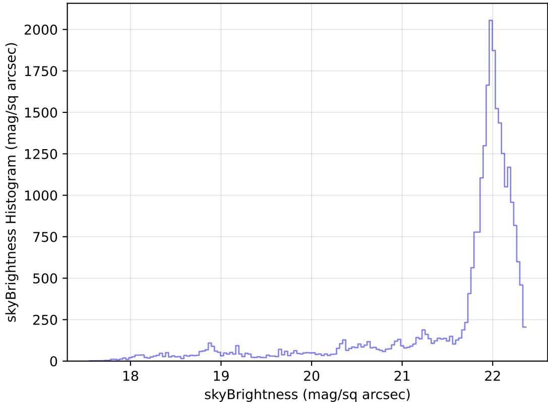
too_elab_heavy_r128_d2_gz_v3.4_10yrs Yr 1 g band: skyBrightness Histogram
