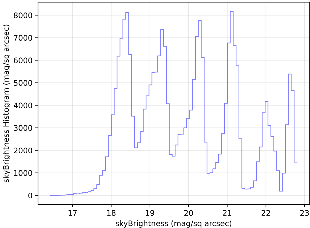
too_elab_heavy_r128_d2_gz_v3.4_10yrs Yr 1 all bands: skyBrightness Histogram
