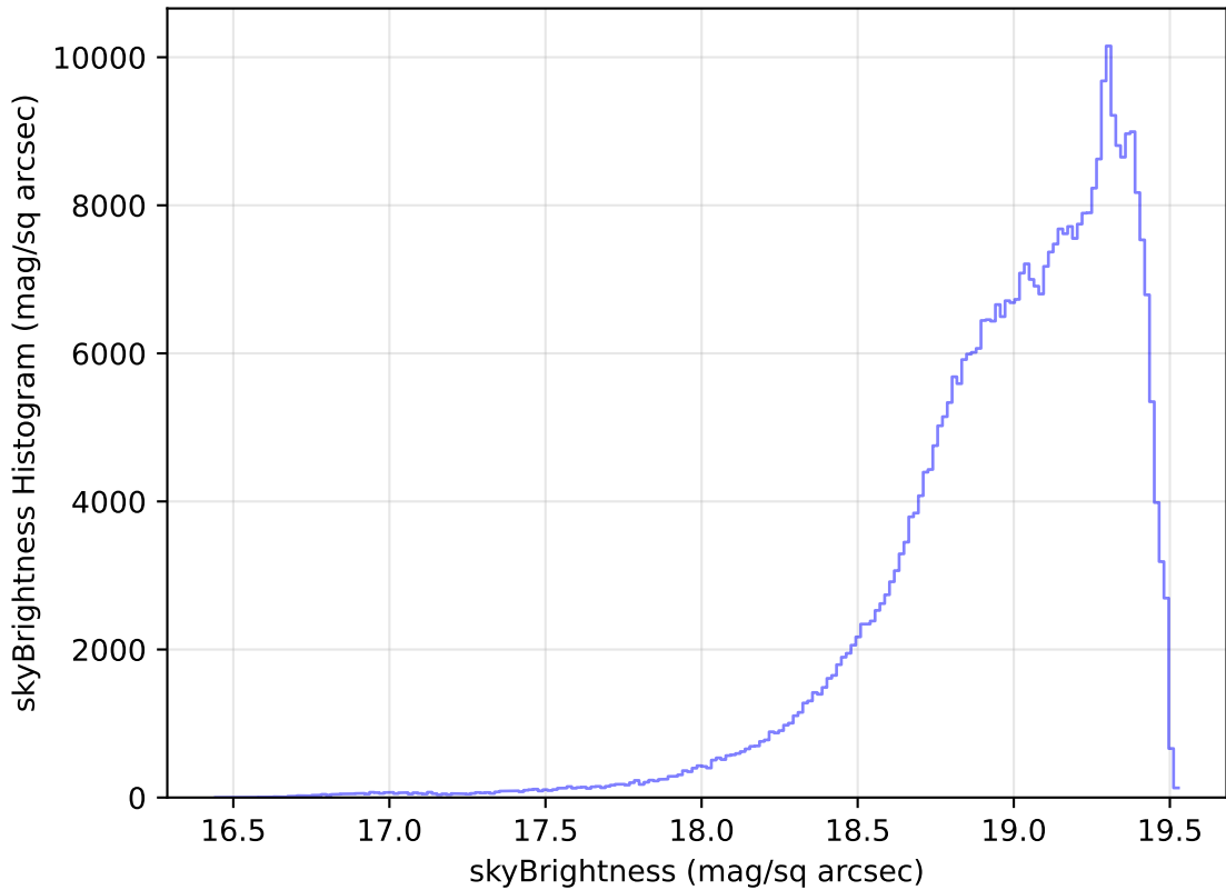
too_elab_heavy_r128_d2_gz_v3.4_10yrs WFD z band: skyBrightness Histogram
