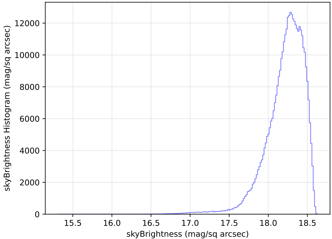
too_elab_heavy_r128_d2_gz_v3.4_10yrs WFD y band: skyBrightness Histogram
