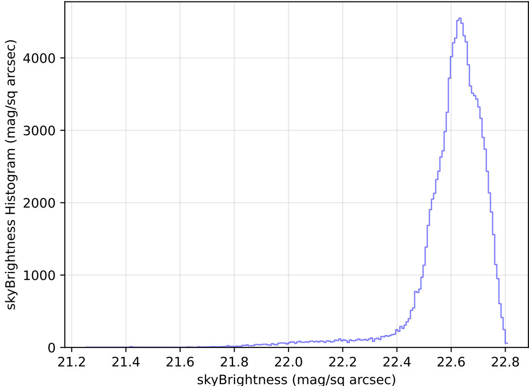
too_elab_heavy_r128_d2_gz_v3.4_10yrs WFD u band: skyBrightness Histogram
