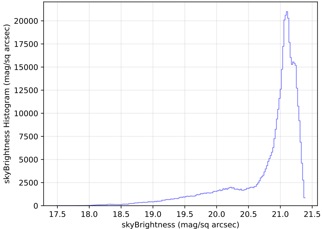
too_elab_heavy_r128_d2_gz_v3.4_10yrs WFD r band: skyBrightness Histogram
