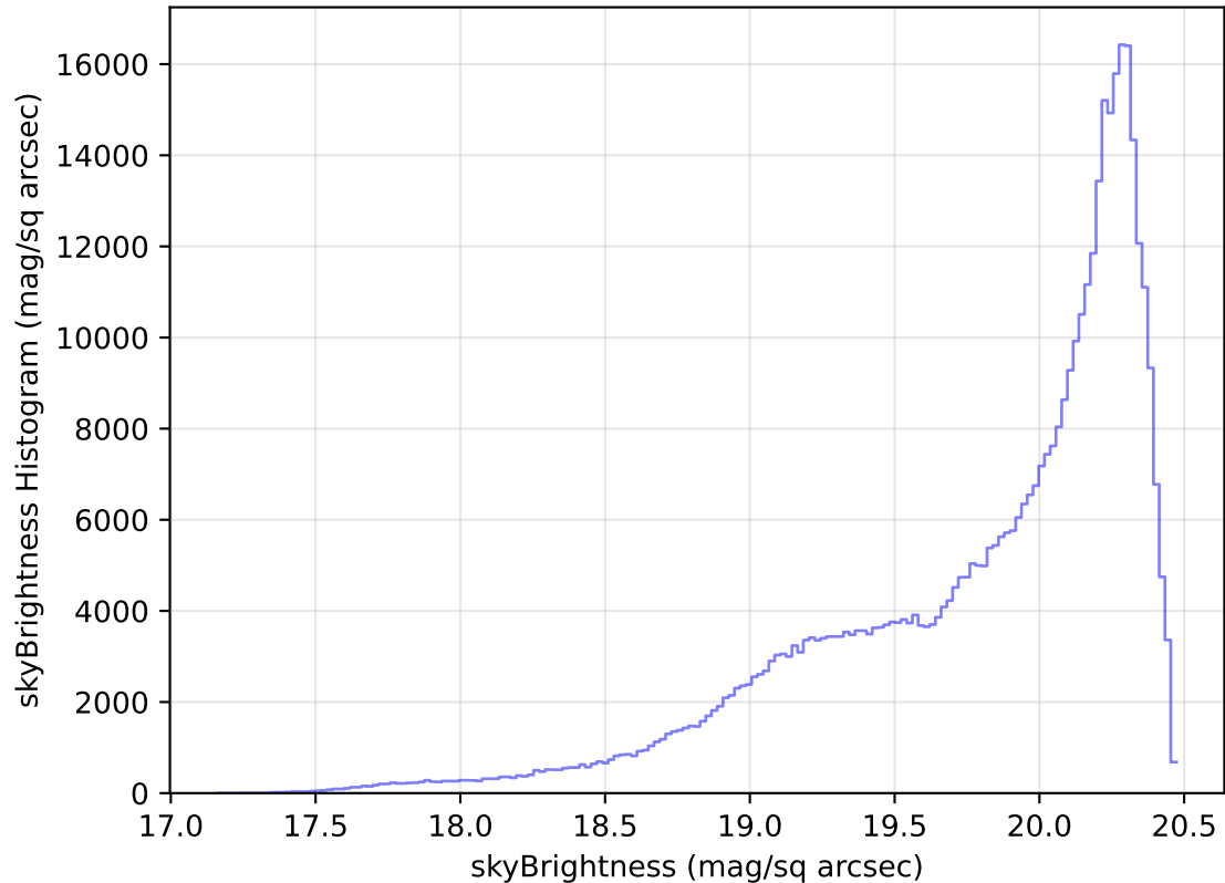
too_elab_heavy_r128_d2_gz_v3.4_10yrs WFD i band: skyBrightness Histogram
