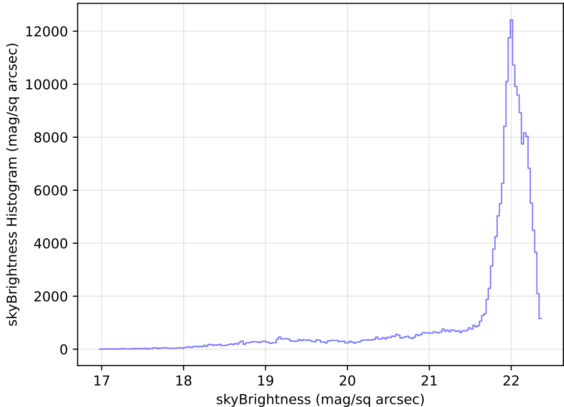
too_elab_heavy_r128_d2_gz_v3.4_10yrs WFD g band: skyBrightness Histogram
