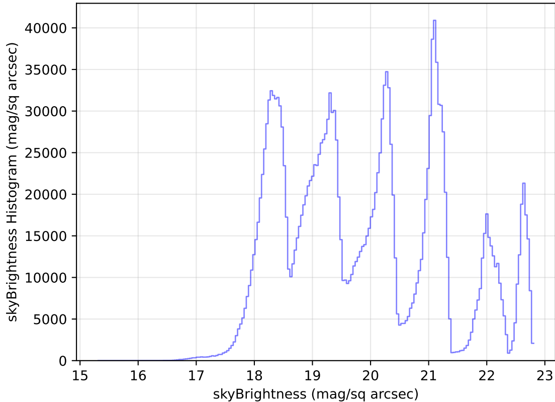
too_elab_heavy_r128_d2_gz_v3.4_10yrs WFD all bands: skyBrightness Histogram
