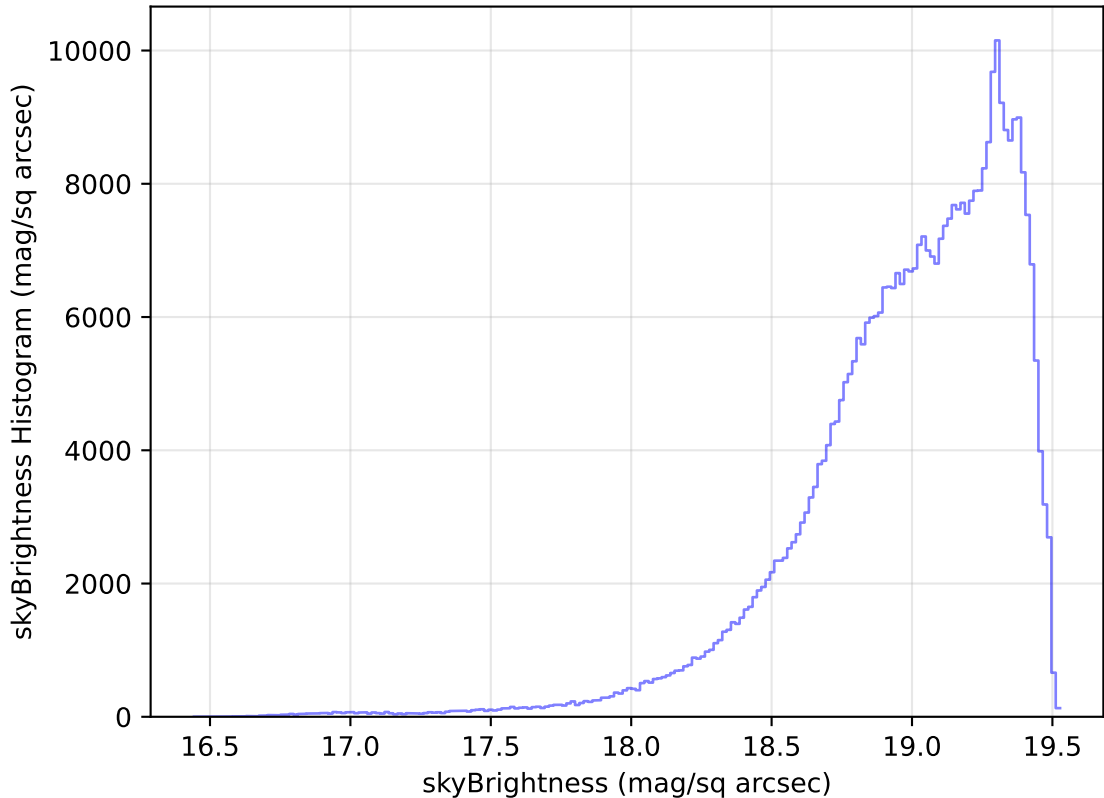
too_elab_heavy_r128_d2_gz_v3.4_10yrs All sky z band: skyBrightness Histogram
