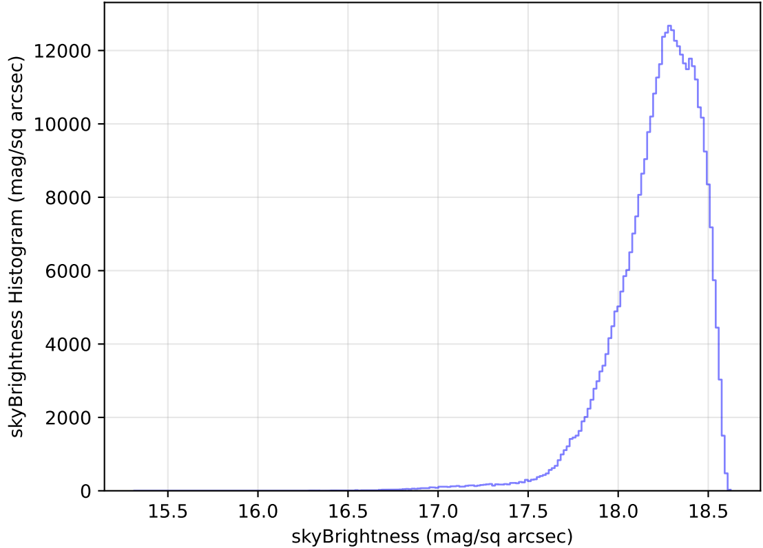
too_elab_heavy_r128_d2_gz_v3.4_10yrs All sky y band: skyBrightness Histogram
