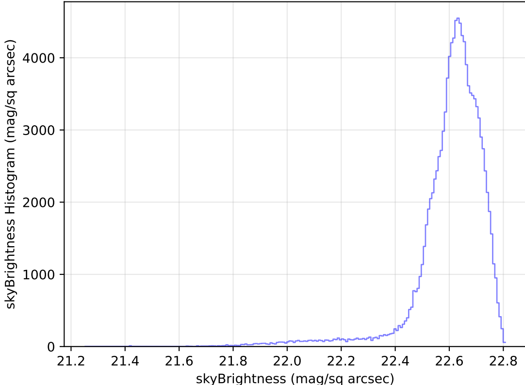
too_elab_heavy_r128_d2_gz_v3.4_10yrs All sky u band: skyBrightness Histogram
