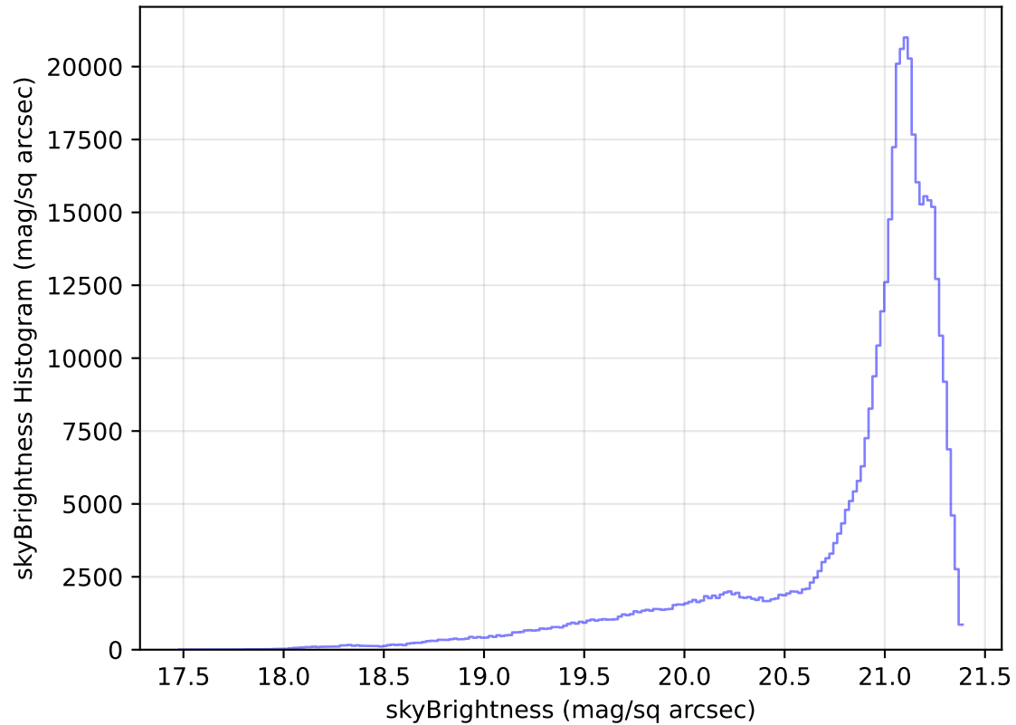
too_elab_heavy_r128_d2_gz_v3.4_10yrs All sky r band: skyBrightness Histogram
