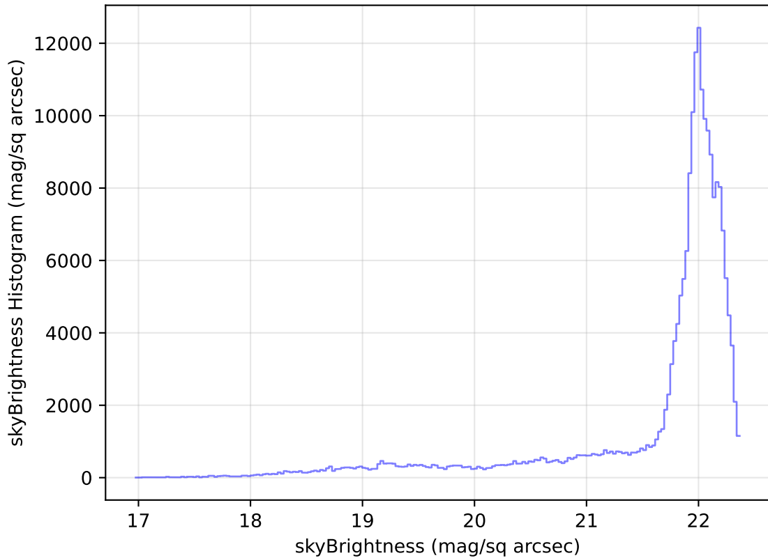
too_elab_heavy_r128_d2_gz_v3.4_10yrs All sky g band: skyBrightness Histogram
