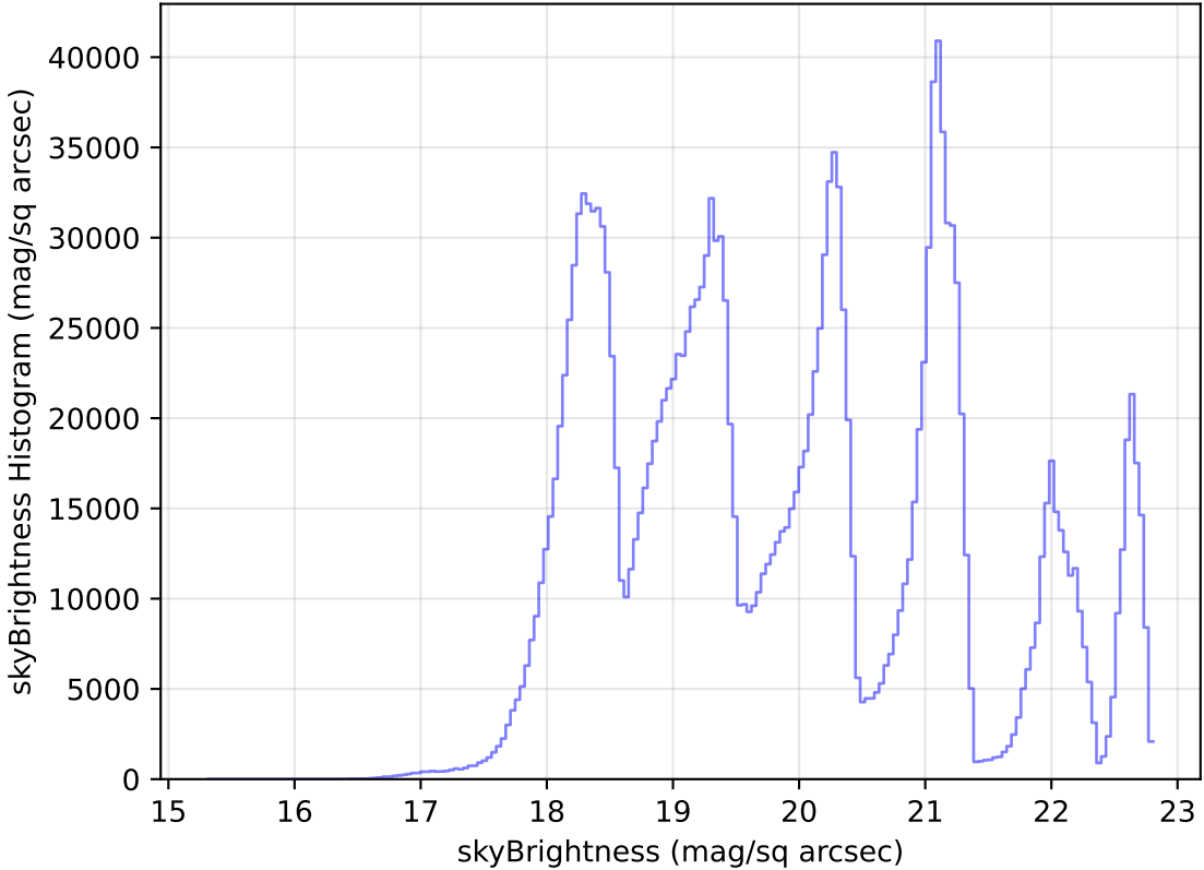
too_elab_heavy_r128_d2_gz_v3.4_10yrs All sky all bands: skyBrightness Histogram
