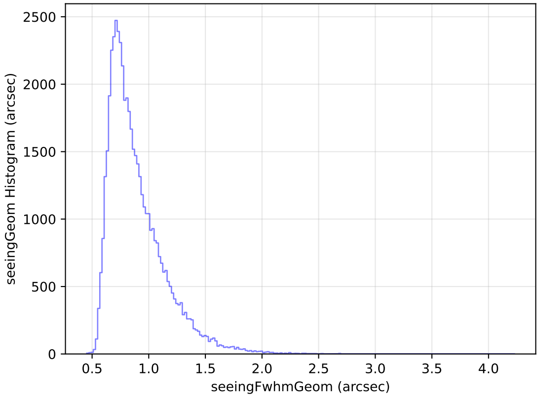
too_elab_heavy_r128_d2_gz_v3.4_10yrs Yr 1 r band: seeingGeom Histogram
