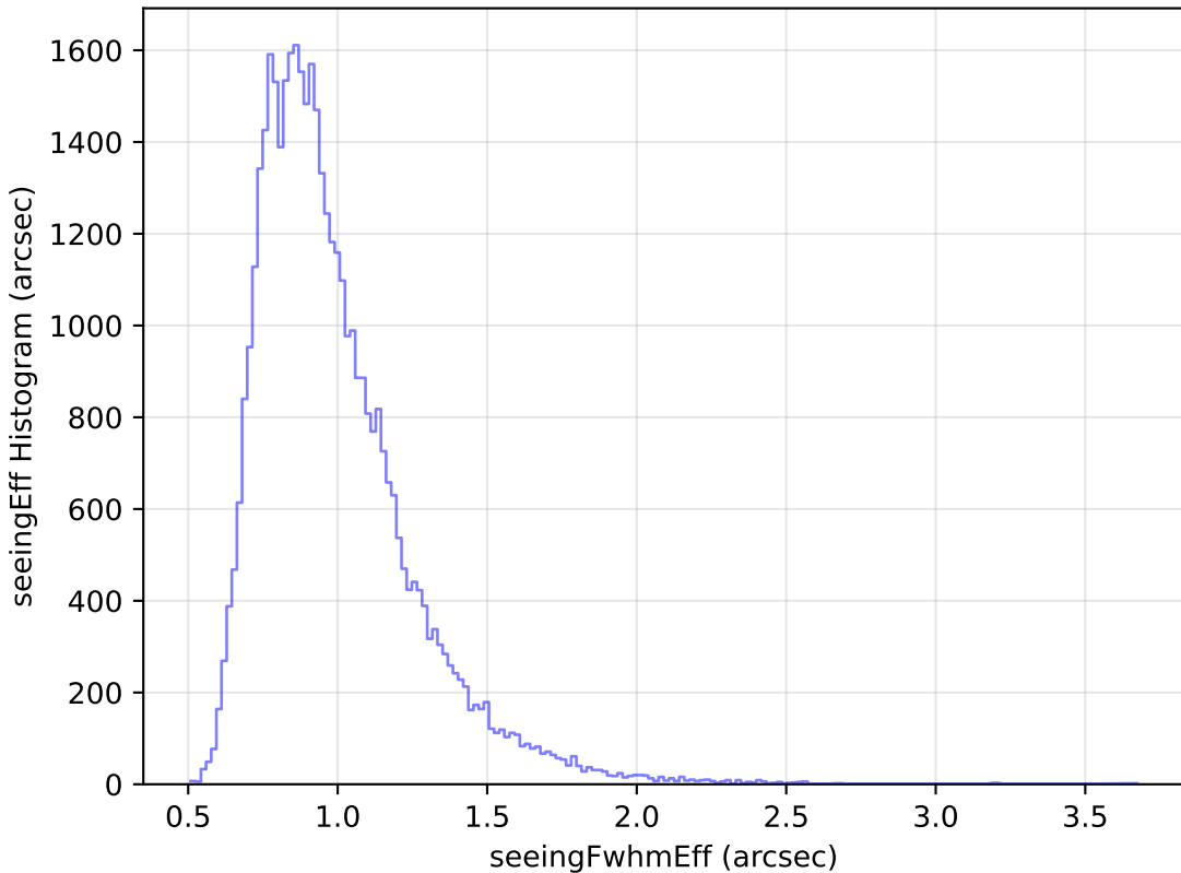
too_elab_heavy_r128_d2_gz_v3.4_10yrs Yr 1 z band: seeingEff Histogram
