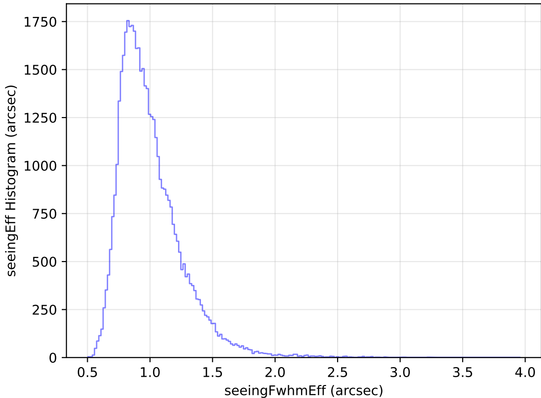
too_elab_heavy_r128_d2_gz_v3.4_10yrs Yr 1 y band: seeingEff Histogram
