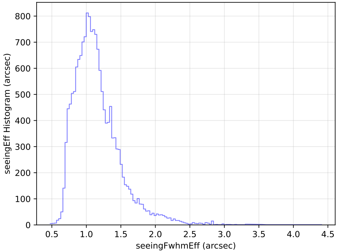
too_elab_heavy_r128_d2_gz_v3.4_10yrs Yr 1 u band: seeingEff Histogram
