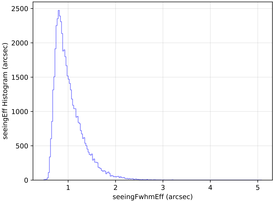
too_elab_heavy_r128_d2_gz_v3.4_10yrs Yr 1 r band: seeingEff Histogram
