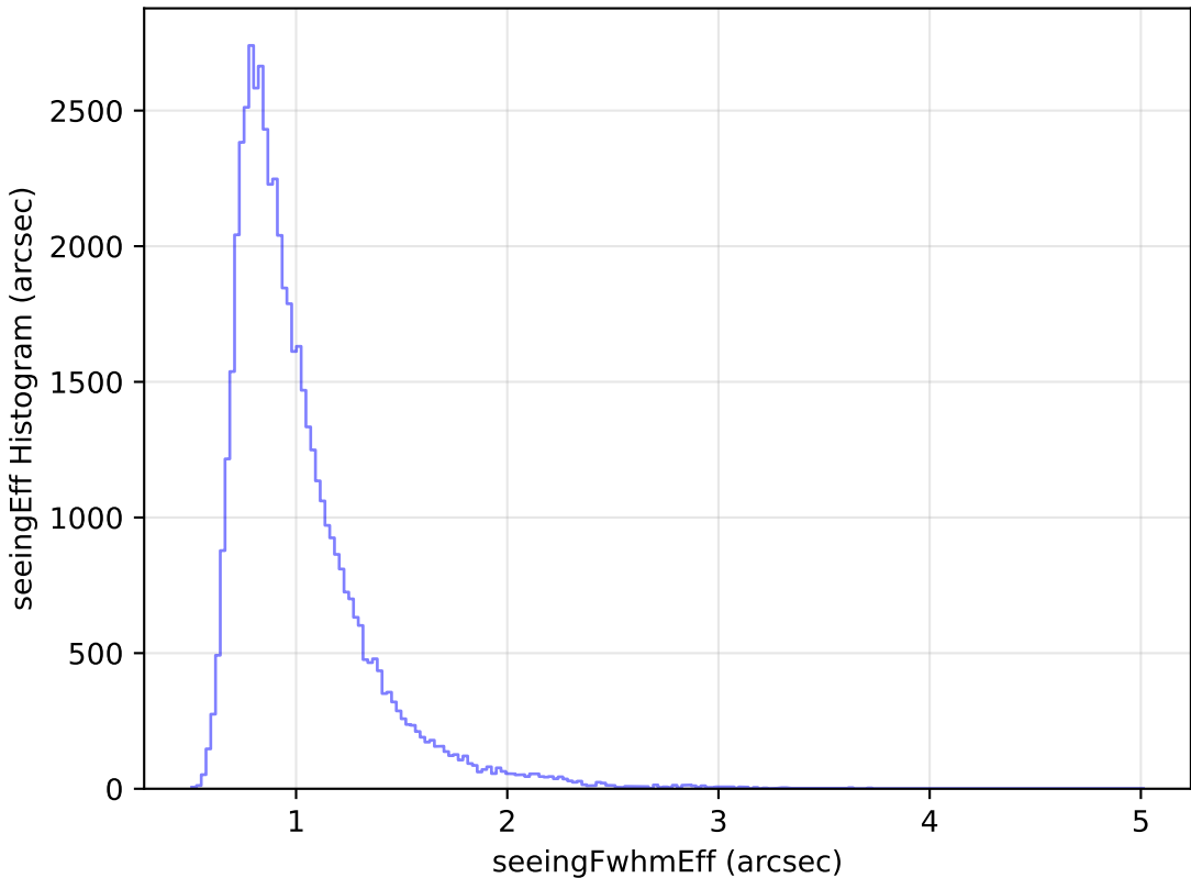
too_elab_heavy_r128_d2_gz_v3.4_10yrs Yr 1 i band: seeingEff Histogram
