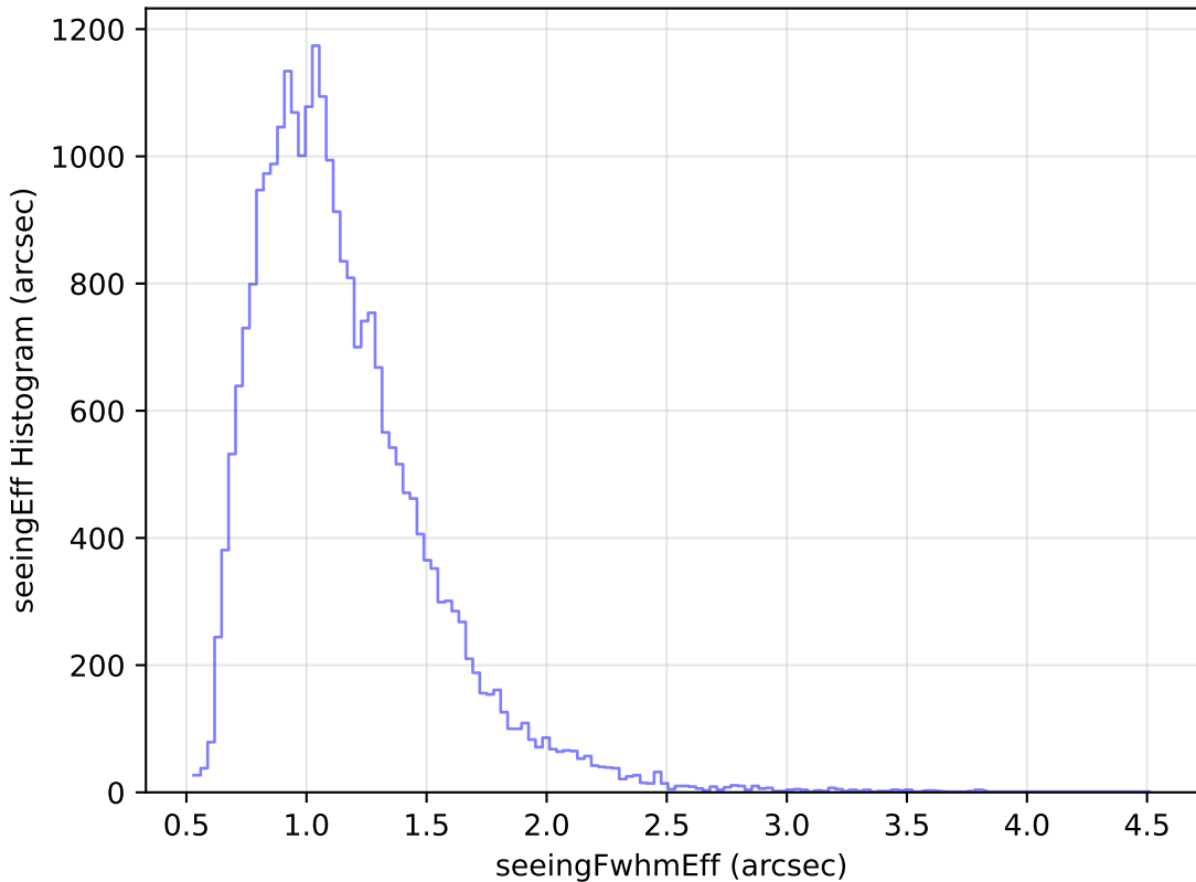
too_elab_heavy_r128_d2_gz_v3.4_10yrs Yr 1 g band: seeingEff Histogram
