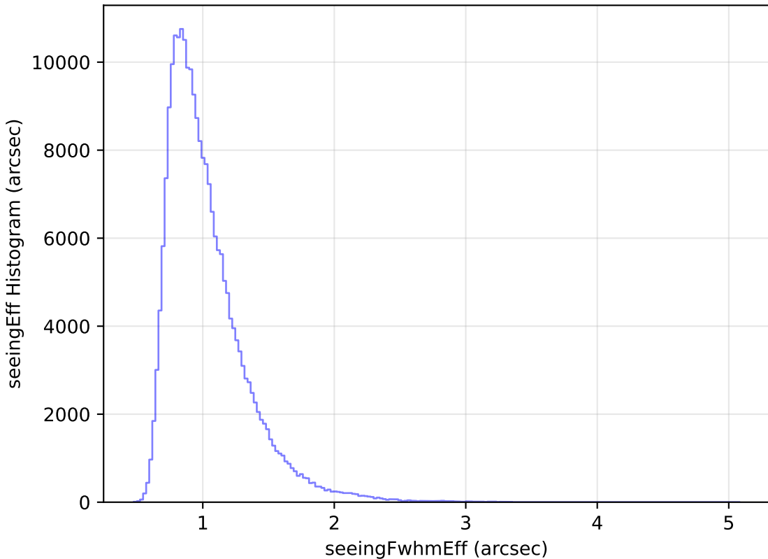
too_elab_heavy_r128_d2_gz_v3.4_10yrs Yr 1 all bands: seeingEff Histogram
