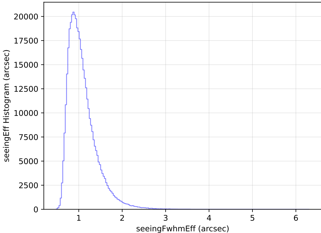
too_elab_heavy_r128_d2_gz_v3.4_10yrs WFD z band: seeingEff Histogram
