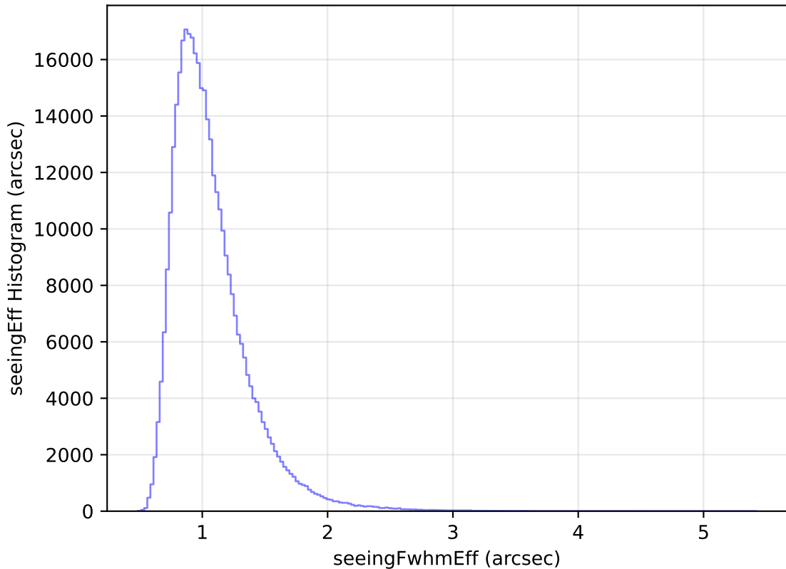
too_elab_heavy_r128_d2_gz_v3.4_10yrs WFD y band: seeingEff Histogram
