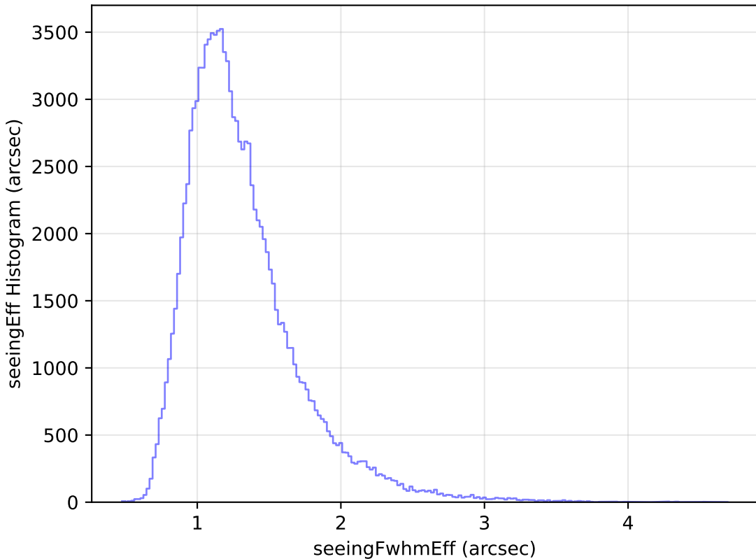
too_elab_heavy_r128_d2_gz_v3.4_10yrs WFD u band: seeingEff Histogram
