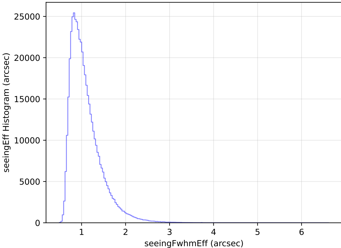
too_elab_heavy_r128_d2_gz_v3.4_10yrs WFD i band: seeingEff Histogram
