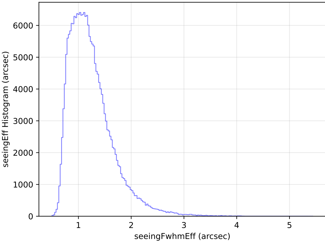
too_elab_heavy_r128_d2_gz_v3.4_10yrs WFD g band: seeingEff Histogram
