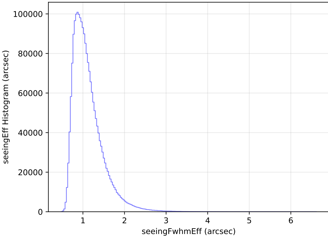
too_elab_heavy_r128_d2_gz_v3.4_10yrs WFD all bands: seeingEff Histogram
