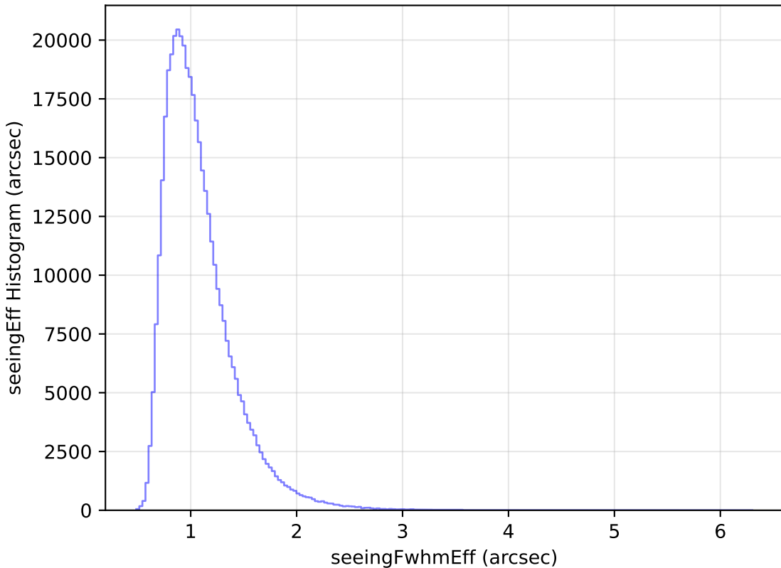
too_elab_heavy_r128_d2_gz_v3.4_10yrs All sky z band: seeingEff Histogram
