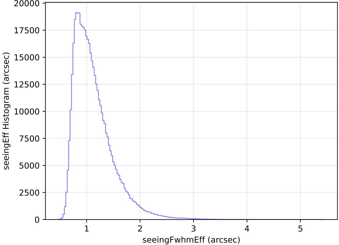
too_elab_heavy_r128_d2_gz_v3.4_10yrs All sky r band: seeingEff Histogram
