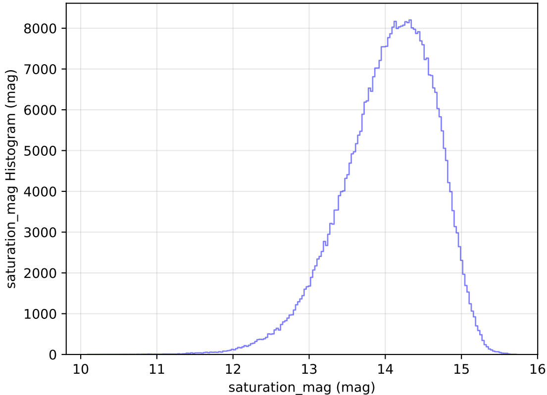
too_elab_heavy_r128_d2_gz_v3.4_10yrs WFD z band: saturation_mag Histogram
