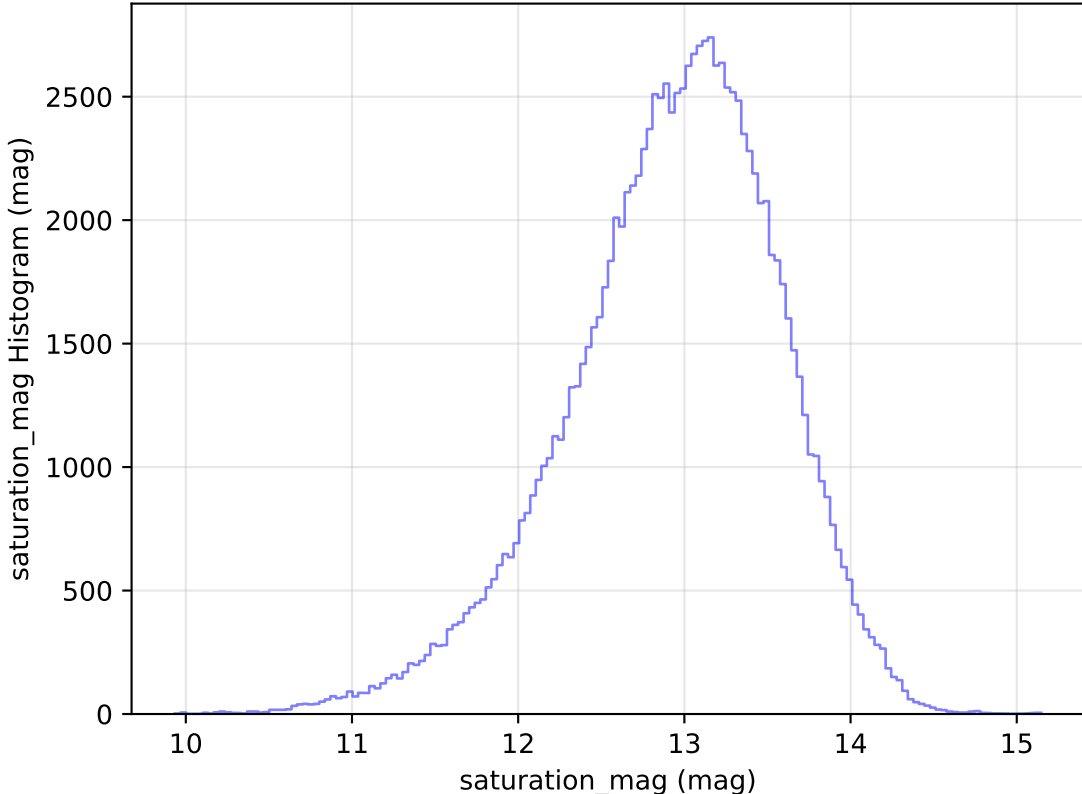
too_elab_heavy_r128_d2_gz_v3.4_10yrs WFD u band: saturation_mag Histogram
