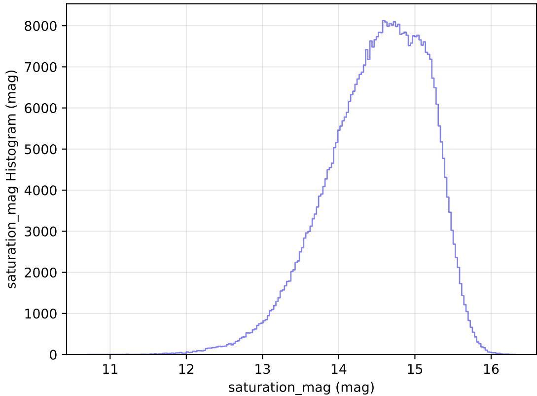
too_elab_heavy_r128_d2_gz_v3.4_10yrs WFD r band: saturation_mag Histogram
