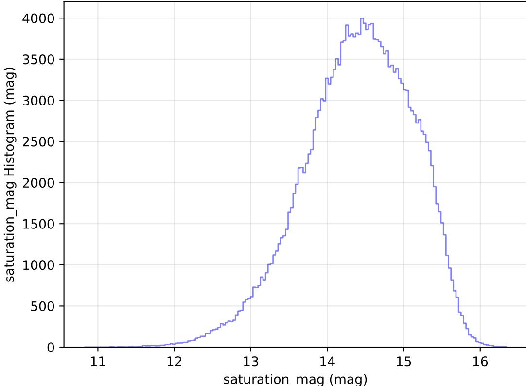
too_elab_heavy_r128_d2_gz_v3.4_10yrs WFD g band: saturation_mag Histogram
