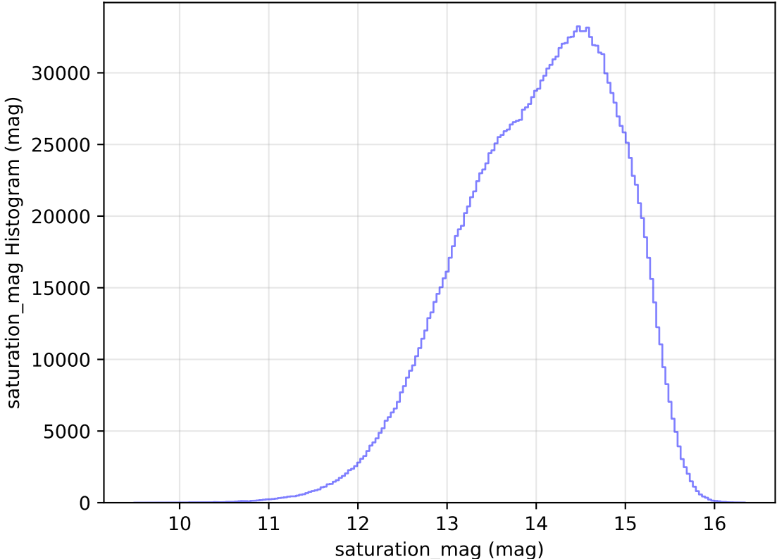
too_elab_heavy_r128_d2_gz_v3.4_10yrs WFD all bands: saturation_mag Histogram
