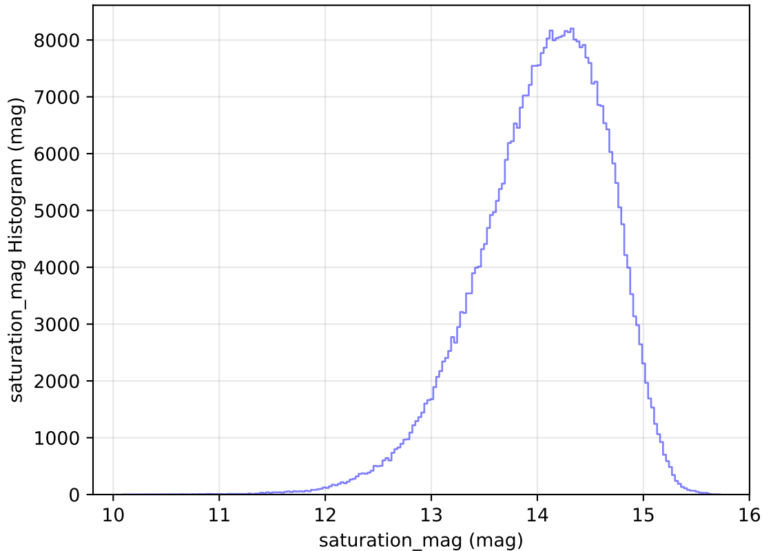
too_elab_heavy_r128_d2_gz_v3.4_10yrs All sky z band: saturation_mag Histogram
